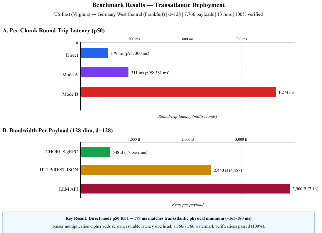
FIG. 8 Benchmark Results: Transatlantic Latency Distribution and Bandwidth vs. Existing Protocols
